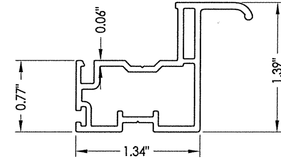
8 LIFT RAIL
