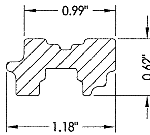
15 STILE/RAIL REINFORCEMENT
