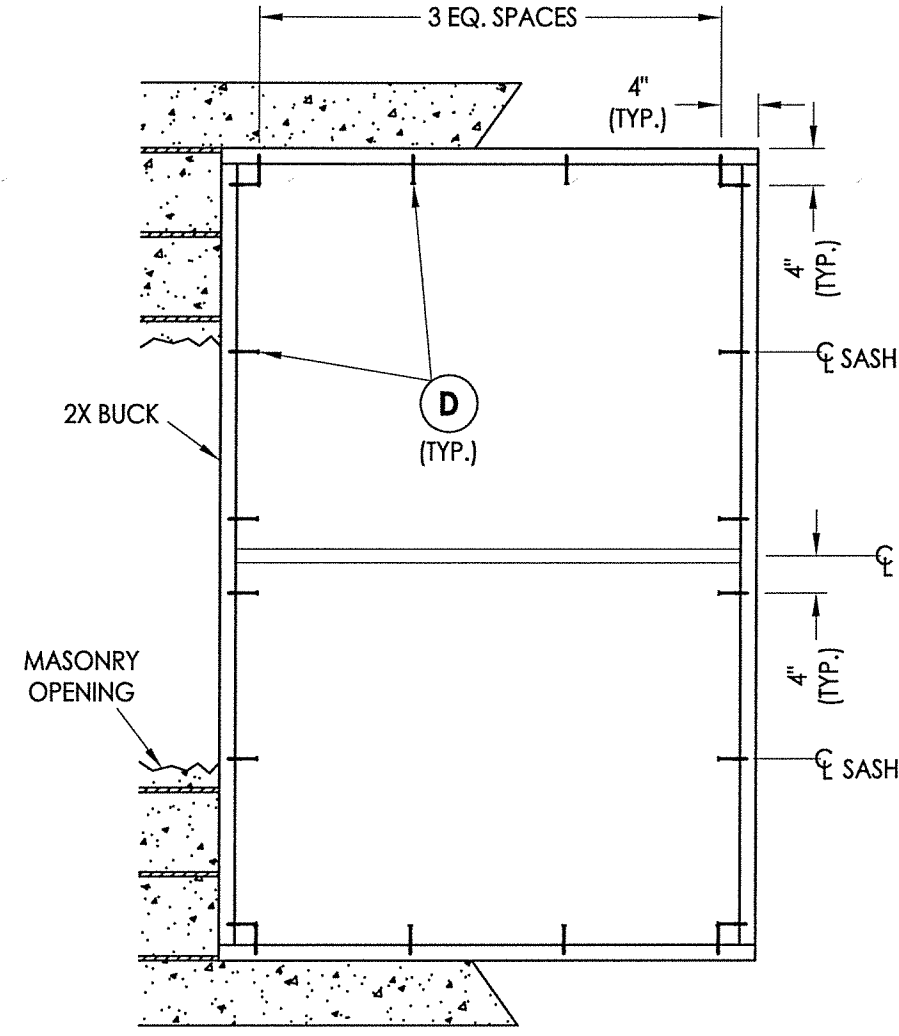
BUCK ANCHORING
