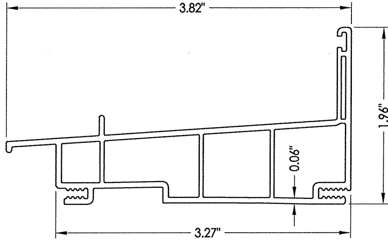
4 SILL
