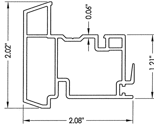
6 FIXED MEETING RAIL
